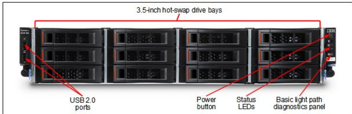
Figure 3. Front view of the System x3630 M4 with twelve drive bays
